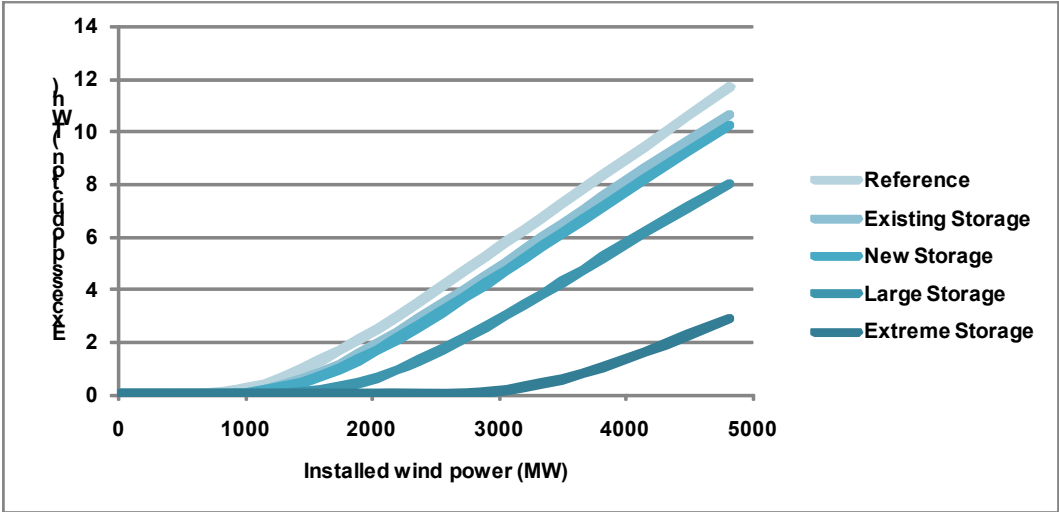
Figure 2.2.1. Installed wind power and excess electricity production in an open energy system analysis of the reference energy system without PHS and with different sizes of PHS.
